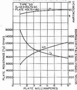
AVERAGE PLATE CHARACTERISTICS
