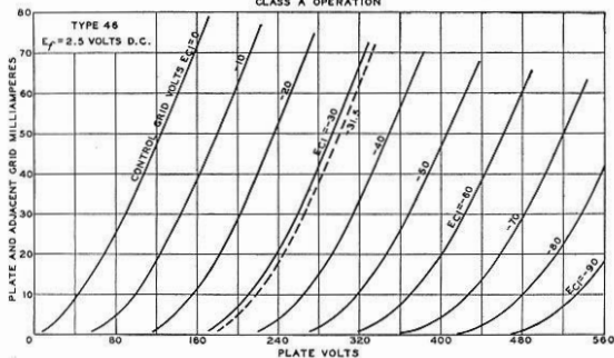
AVERAGE PLATE CHARACTERISTICS CLASS A OPERATION
