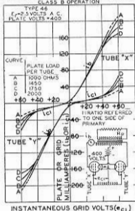
DYNAMIC TRANSFER CHARACTERISTICS CLASS B OPERATION
