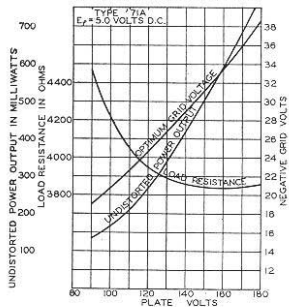
AVERAGE CHARACTERISTICS
