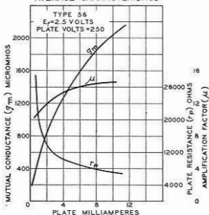
AVERAGE CHARACTERISTICS
