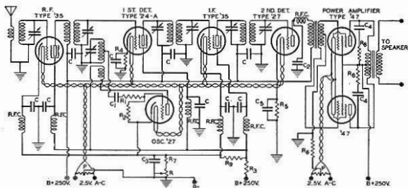
TYPICAL SUPERHETERODYNE RECEIVER FOR A-C OPERATION
