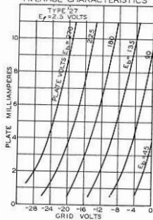
AVERAGE CHARACTERISTICS
