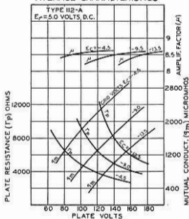
AVERAGE CHARACTERISTICS
