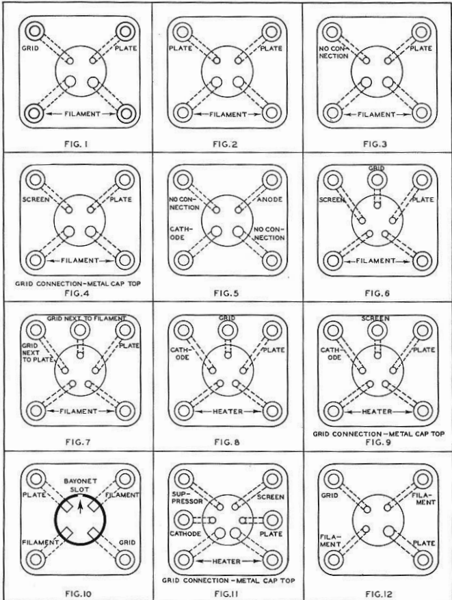
TOP VIEWS OF SOCKETS
