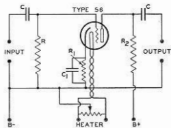
RESISTANCE-COUPLED A-F AMPLIFIER
