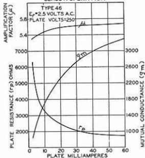
AVERAGE CHARACTERISTICS CLASS A OPERATION
