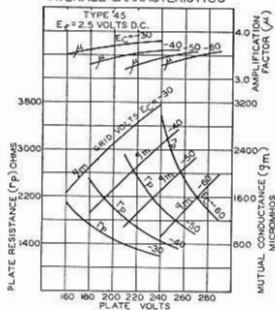
AVERAGE CHARACTERISTICS
