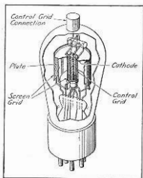
Interior View of '24-A
