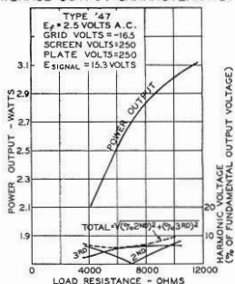
AVERAGE OUTPUT CHARACTERISTICS
