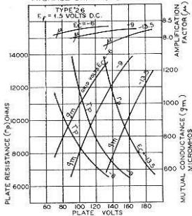
AVERAGE CHARACTERISTICS
