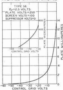
AVERAGE CHARACTERISTICS
