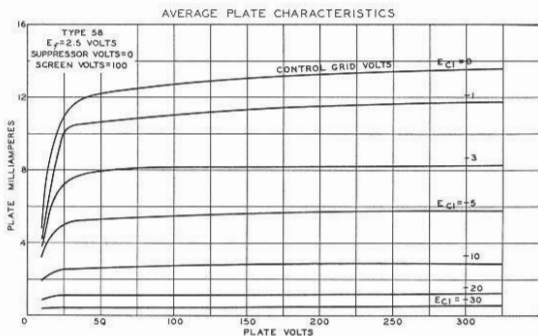
AVERAGE CHARACTERISTICS
