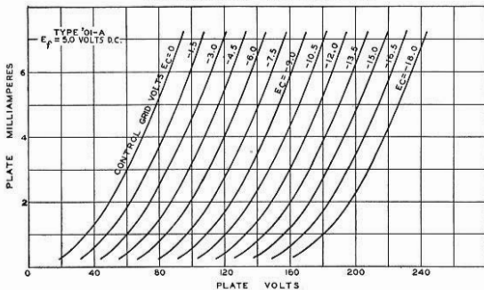
AVERAGE CHARACTERISTICS
