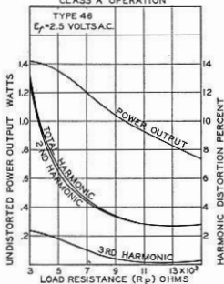
AVERAGE CHARACTERISTICS CLASS A OPERATION
