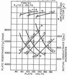
AVERAGE CHARACTERISTICS
