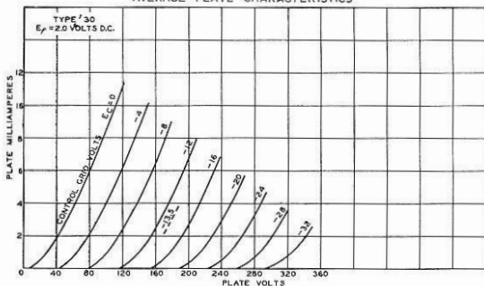
AVERAGE CHARACTERISTICS
