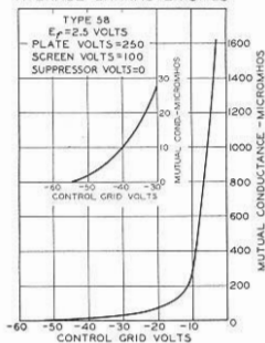
AVERAGE CHARACTERISTICS
