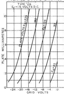
AVERAGE CHARACTERISTICS
