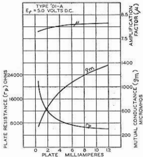
AVERAGE PLATE CHARACTERISTICS
