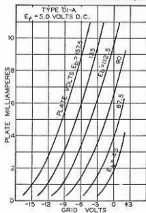
AVERAGE PLATE CHARACTERISTICS
